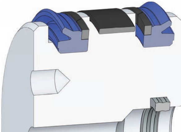
A251 Piston Boğaz Yataklama
